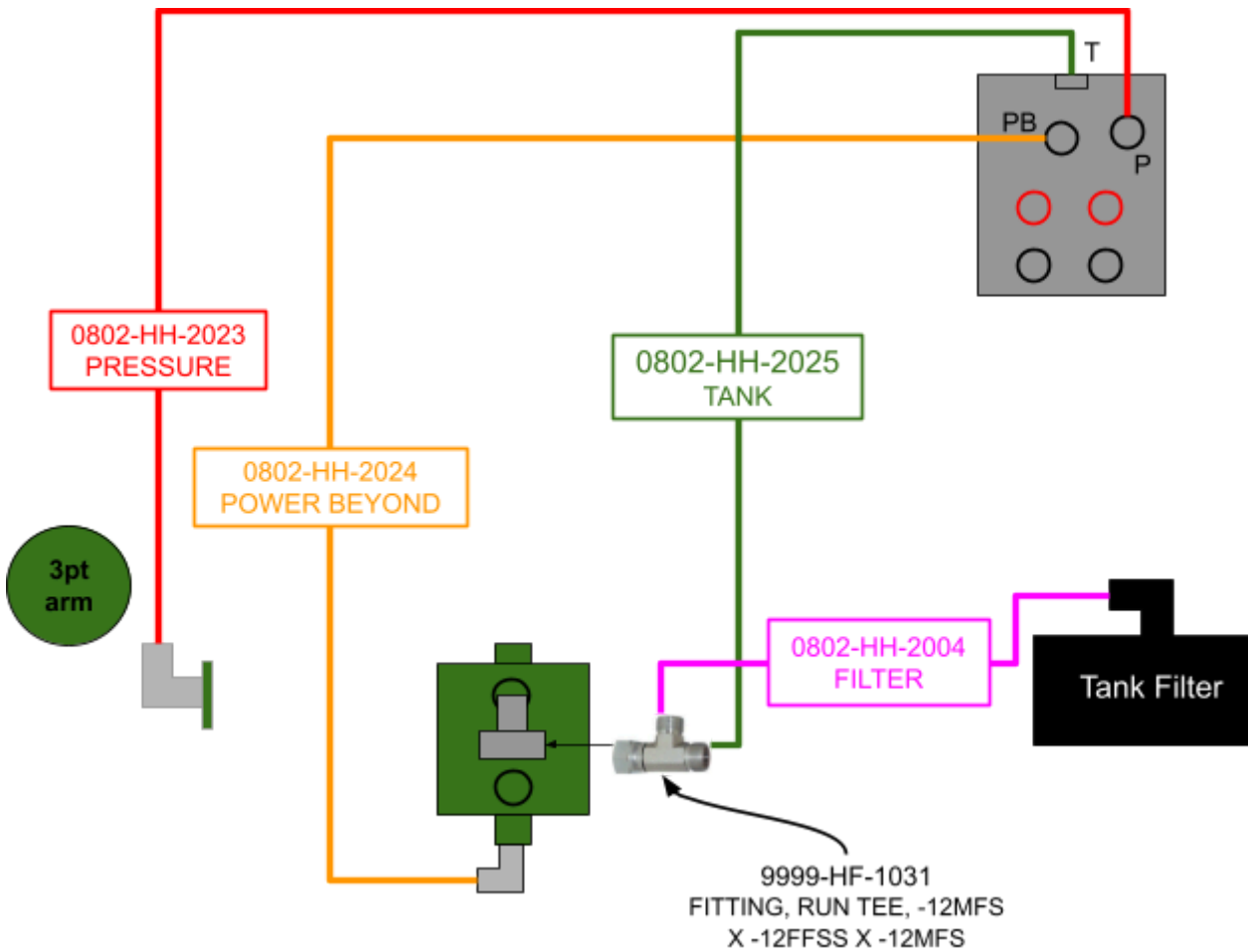
Remote Valve Integration Diagram
